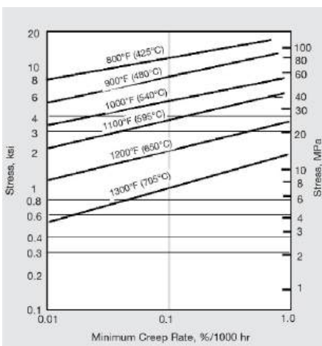
Figure 14 - Typical creep strength of annealed Nickel 201.
